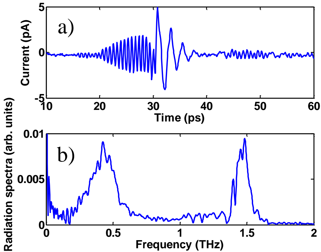
Figure 6-18 : Measured re-radiation waveform in the time domain (top panel) and spectra (bottom panel) for metafilm MM1.
