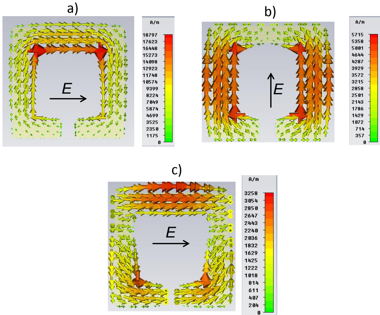
Figure 4-3 Calculated surface current densities for the fundamental LC resonance in part (a) and second order dipole mode in part (b) and third order dipole mode shown in (c)
