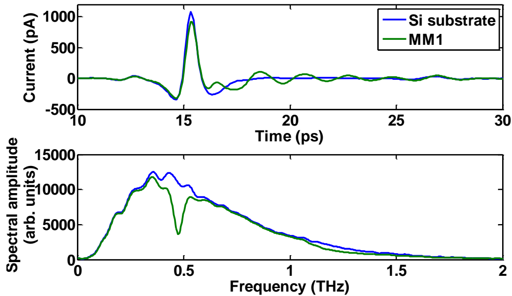
Figure 6-12: Top panel: Measured temporal waveforms for MM1 sample (green) and bare Si reference (blue). Bottom panel: Corresponding transmission spectra.
