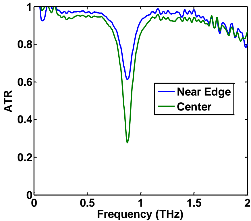
Figure 6-10: Measured reflection (ATR) coefficients of MM3 for the center (blue) and edge (green) beam positions
