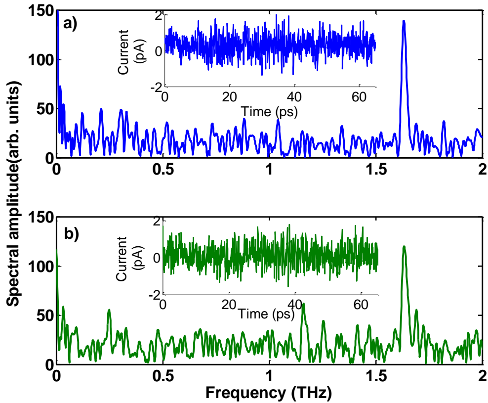
Figure 6-29 Re-radiation measurements on MM3 measured normal to the prism face with inset showing time domain signal. Incident beam near a) the center of the array and b) the array edge.
