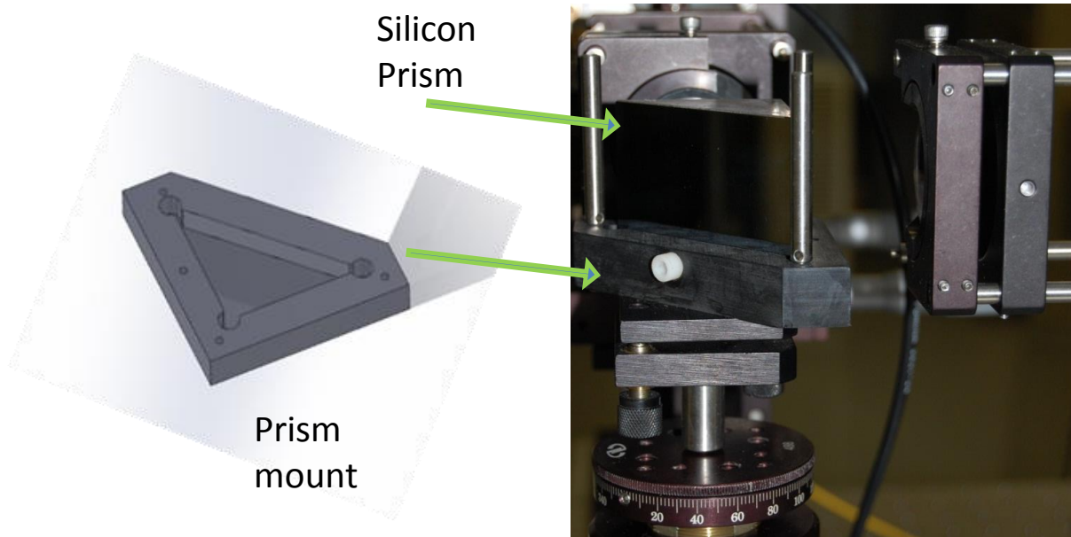
Figure 5-5: Custom Prism mounting assembly.
