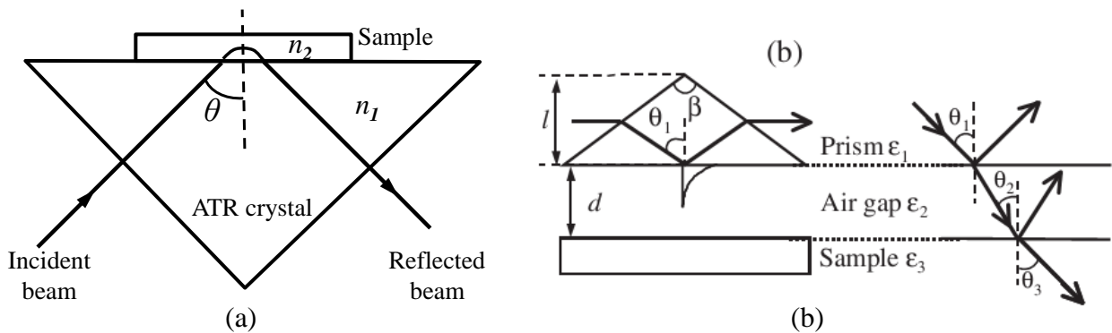
Figure 3-2 Single reflection IRE a) Right angled prism b) Dove prism from [14]
