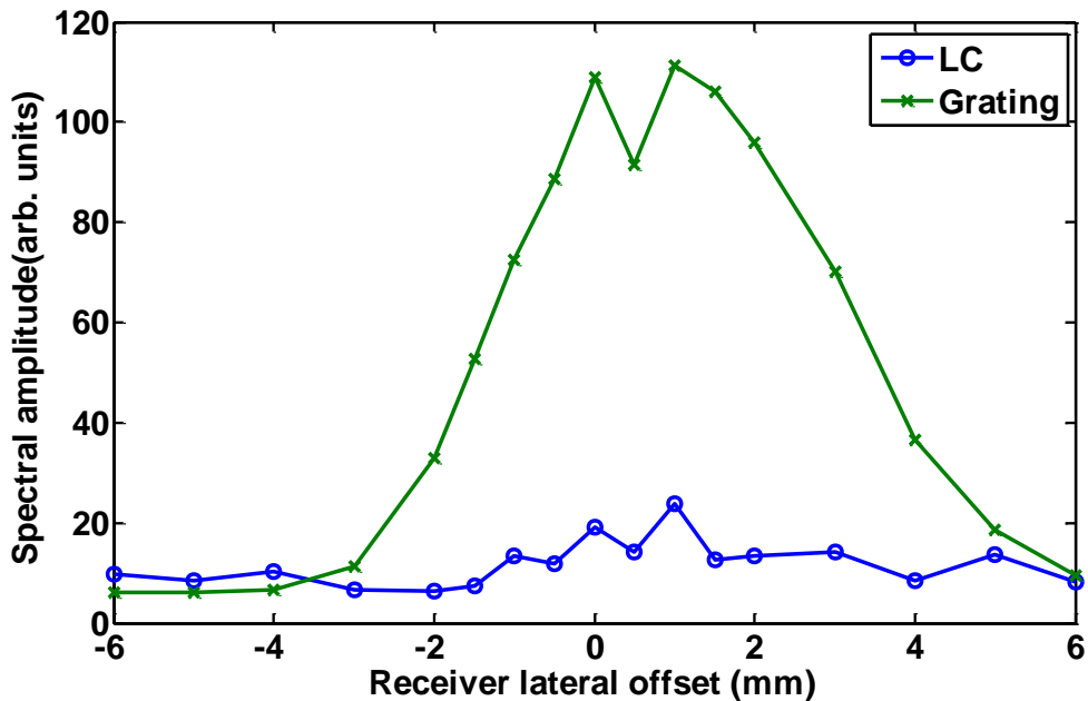
Figure 6-21: Center excited beam profiles from re-radiation waveforms shown here for fundamental LC (blue) and the transmission grating (green) frequencies. Positive offset x is towards the edge and negative offsets x are toward the center of the array (see Figure 6-19).
