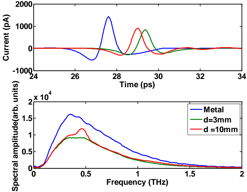
Figure 6-16: Time (top) and frequency (bottom) for THz beam positions on metal (blue), near edge (green: d_{\text{edge}} = 3 mm) and near center (red: d_{\text{edge}} = 10 mm).
