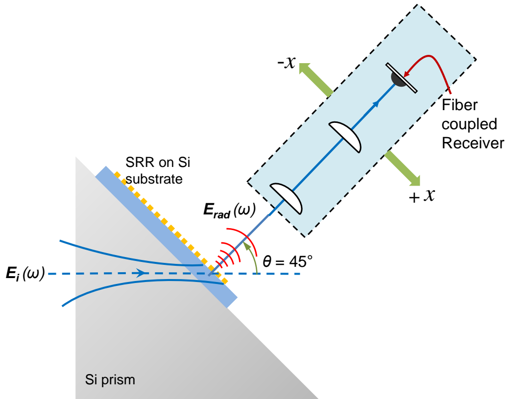
Figure 6-19: Schematic for lateral displacement measurements for re-radiation configuration.
