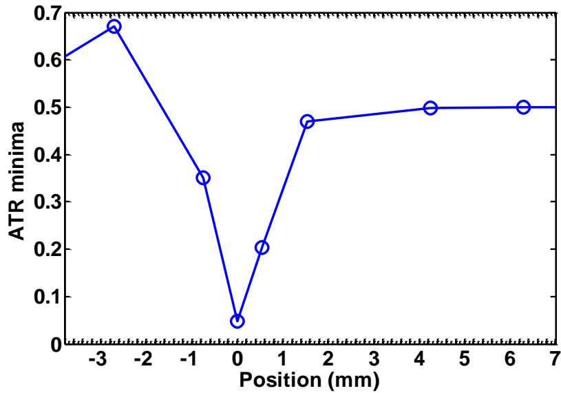
Figure 6-8: Magnitude of the on-resonance reflection coefficient of sample MM1 as a function of the displacement d_{\text{edge}} .
