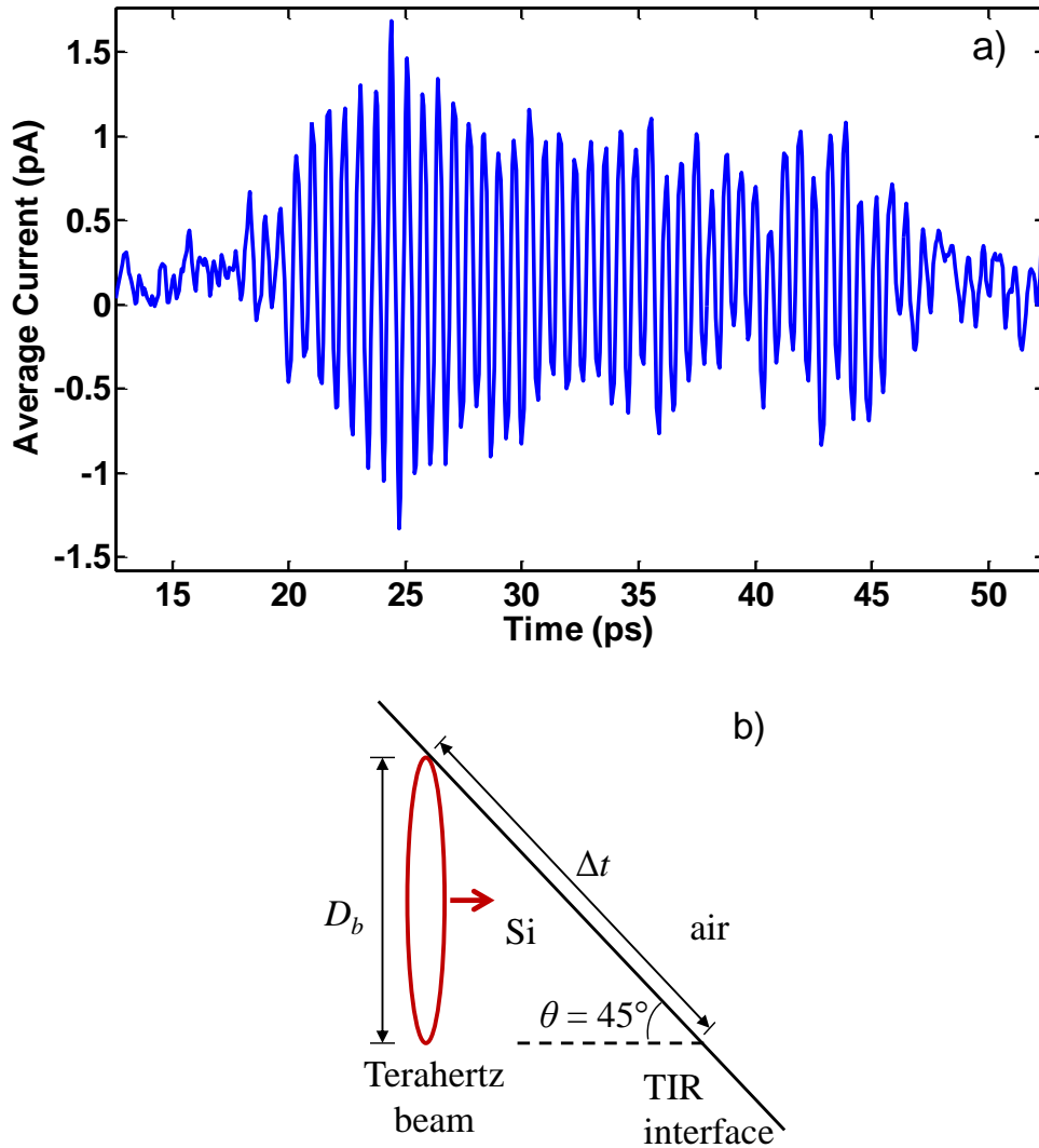
Figure 6-23 a) Transmission grating response from center excited SRR array in the time domain. b) Beam width calculation geometry.
