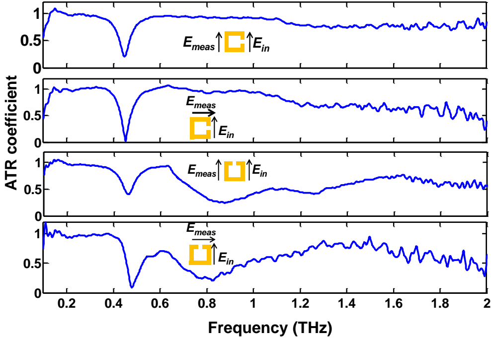
Figure 6-26 ATR spectra for different orientations of the SRR and detector. Incident field is s-polarized.
