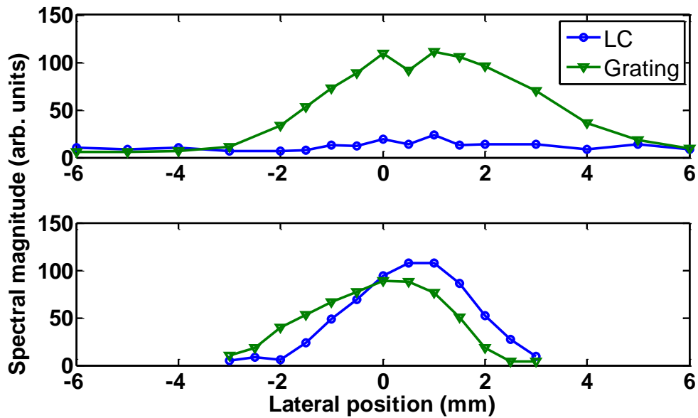
Figure 6-22: Near center (top panel same as Figure 6-21) and near edge (bottom panel same as Figure 6-20) excited beam profile measurements from re-radiation waveforms shown here for fundamental LC (blue) and the transmission grating (green) frequencies. Positive offset is towards the edge and negative offsets are toward the center of the array.
