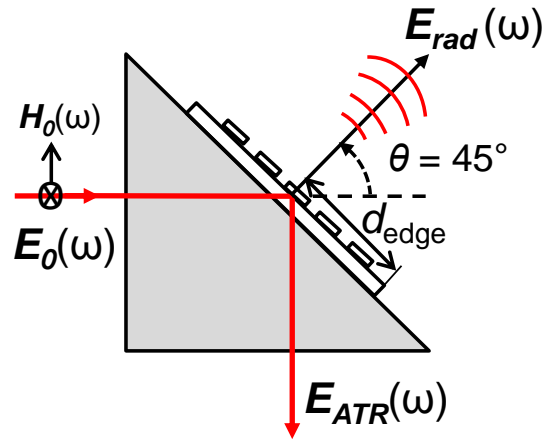
Figure 6-7 Schematic for ATR position dependent measurements.
