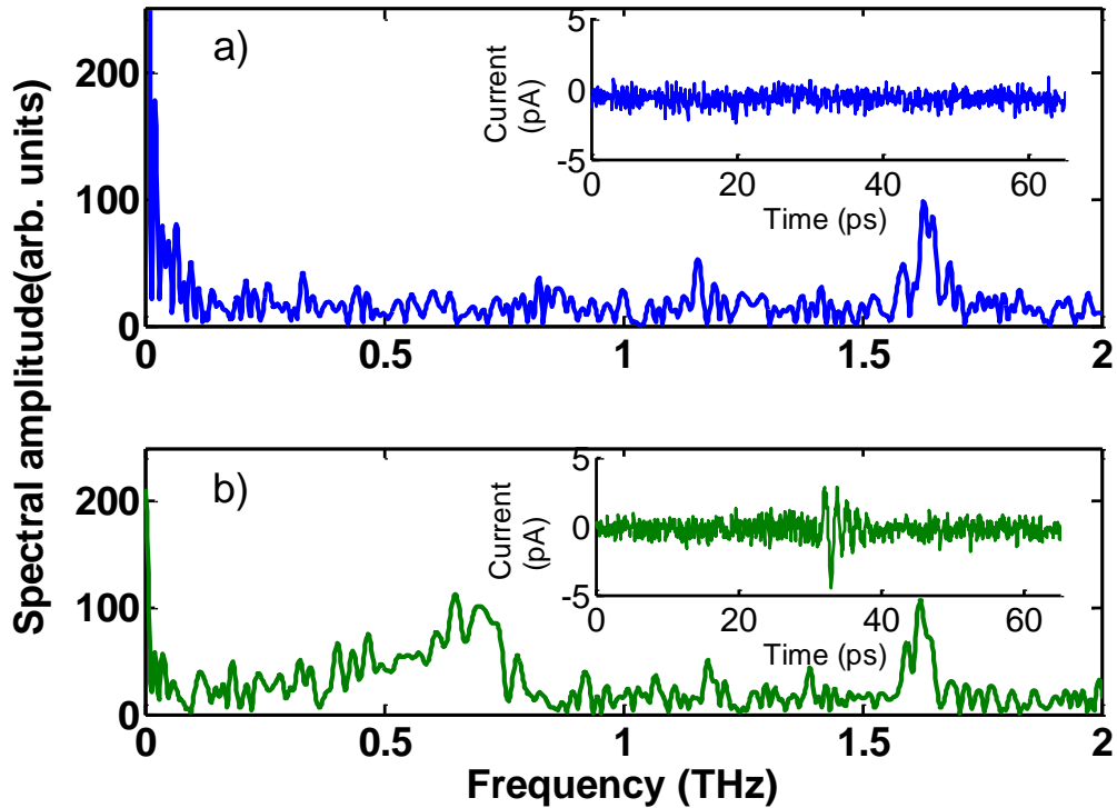
Figure 6-28 Re-radiation measurements on MM2 measured normal to the prism face with inset showing time domain signal. Incident beam a) near the center of the array and b) near the array edge.
