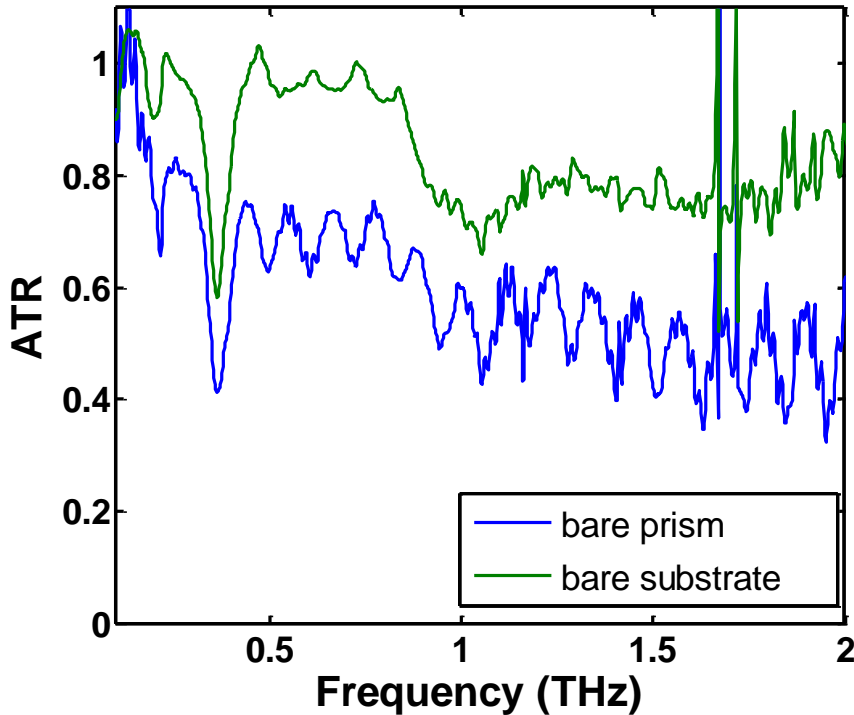
Figure 6-2: Frequency dependent ATR using prism reference (blue) and silicon substrate reference (green).
