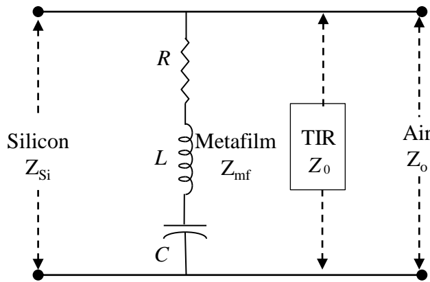
Figure 7-8 Equivalent circuit model for ATR configuration: metafilm on silicon prism.
