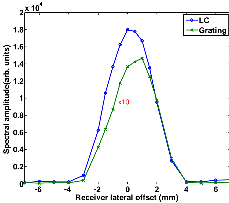
Figure 5-11 Measured beam profile in the confocal configuration as shown in Figure 5-10. The amplitude of the grating frequency profile is x10 for comparison of the beam widths.
