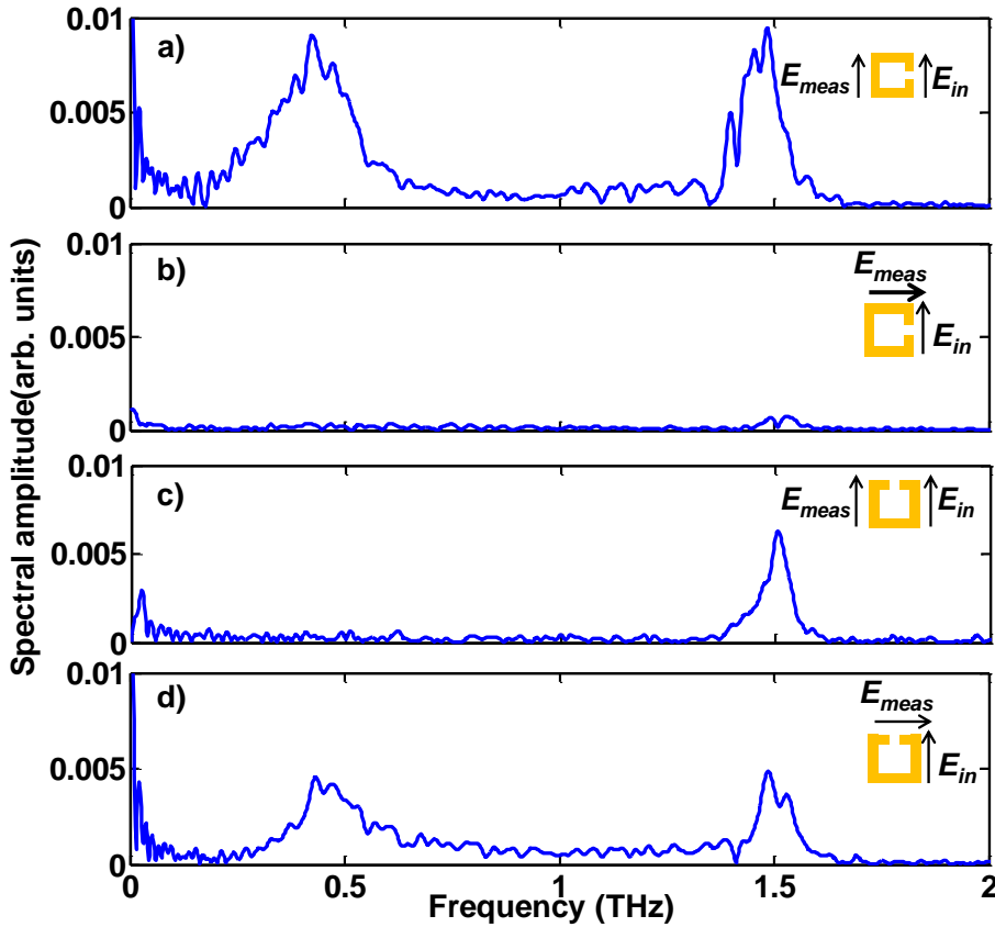
Figure 6-25: Re-radiation spectra for different orientations of the SRR and detector. Incident field is s-polarized.
