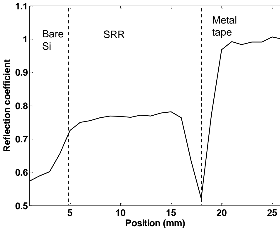
Figure 6-17: Spatially dependent on-resonance (0.45 THz) reflection coefficient for MM1 using reflection THz-TDS
