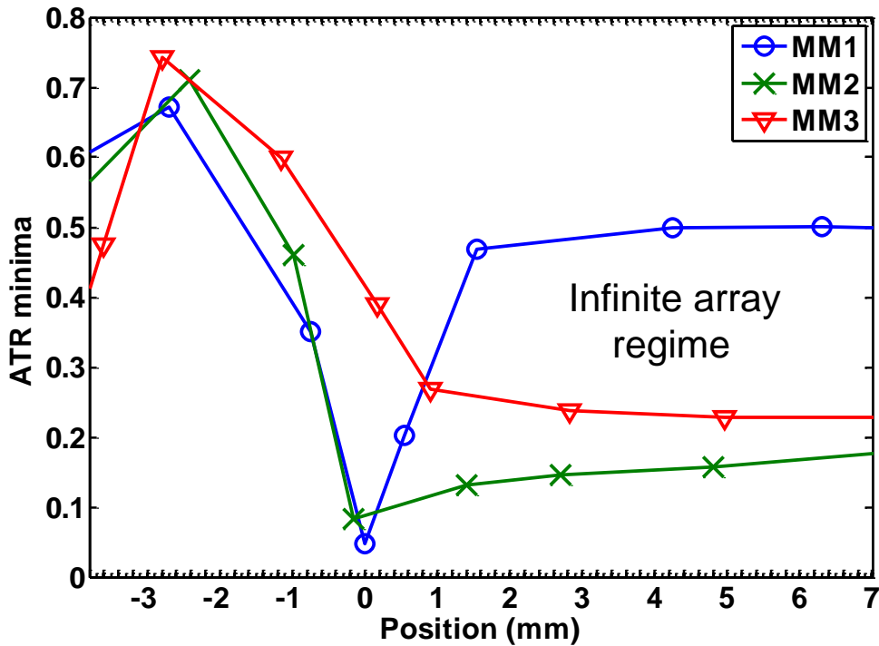
Figure 6-11: Comparison of position dependent on-resonance reflection (ATR) coefficients for MM1, MM2 and MM3.
