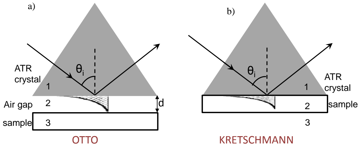
Figure 3-1 ATR geometries a) Otto b) Kretschmann, adapted from [61].
