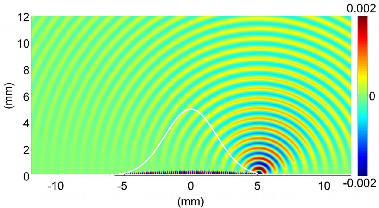
Figure 7-21 Electric field amplitude corresponding to s-polarization at the resonance frequency of 0.4 THz at the TIR boundary for a wire array that is truncated at x = +5 mm. No inter-element coupling is explicitly included in this treatment. The incident terahertz beam is shown in white.[107]
