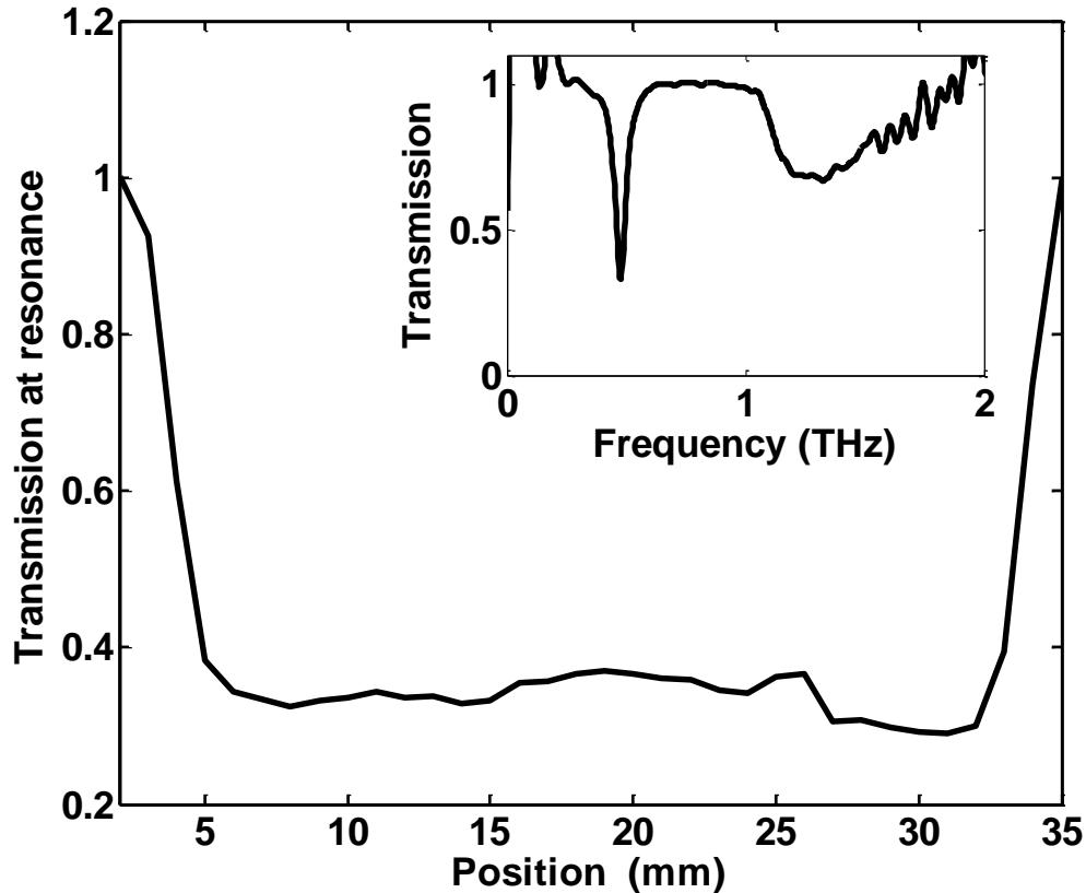
Figure 6-14: Position dependent Transmission (magnitude) at resonance. Inset: Frequency dependent transmission on resonance.
