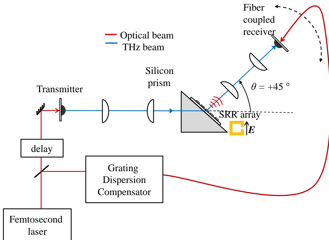
Figure 6-3 Experimental layout to detect re-radiation. Incident electric field polarized as indicated.
