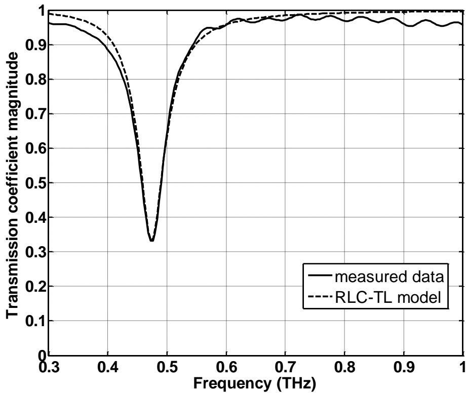
Figure 7-4 Transmission coefficient for metafilm MM1 from measurements (solid) and RLC -TL circuit model (dashed).
