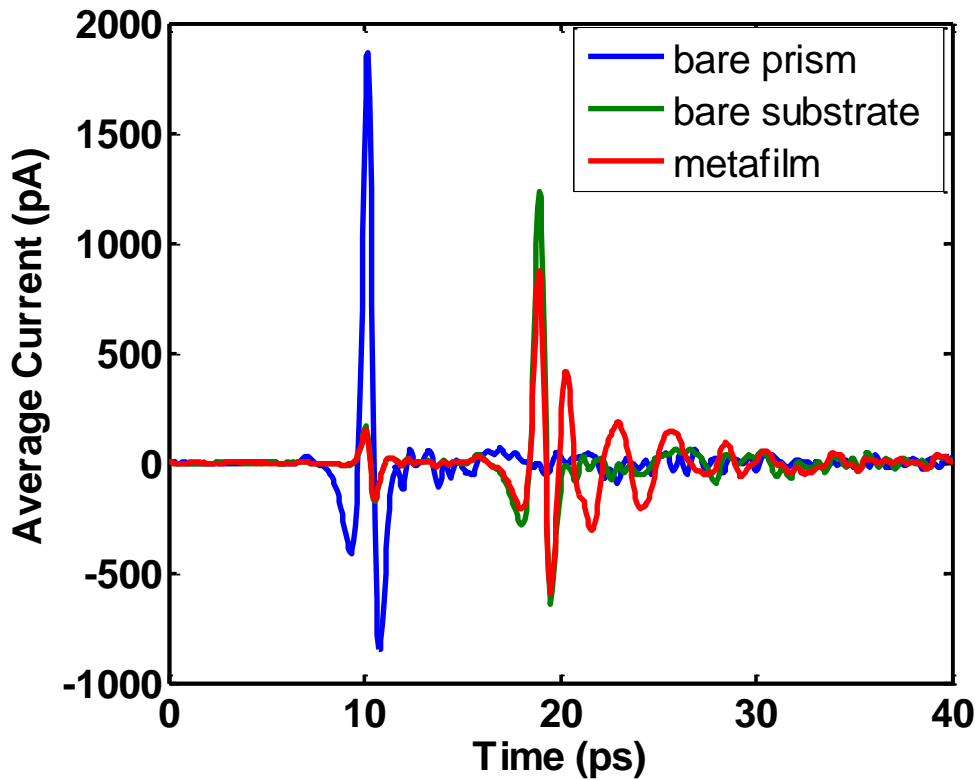
Figure 6-1: Temporal ATR waveforms of bare prism, bare substrate and 1 \text{cm}^2 metafilm sample.
