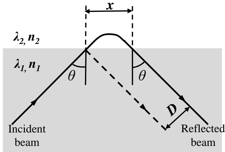
Figure 3-9 Schematic of the Goos-Hanchen shift D on total internal reflection. The dashed line on the reflected side of the normal represents the path taken by the reflected beam as predicted by geometric optics.
