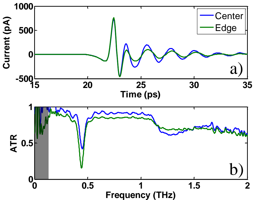
Figure 6-6: Comparison of ATR measurements on sample MM1 for incident beam at the center (blue) and edge (green). a) Reflected terahertz signals and b) ATR coefficients.
