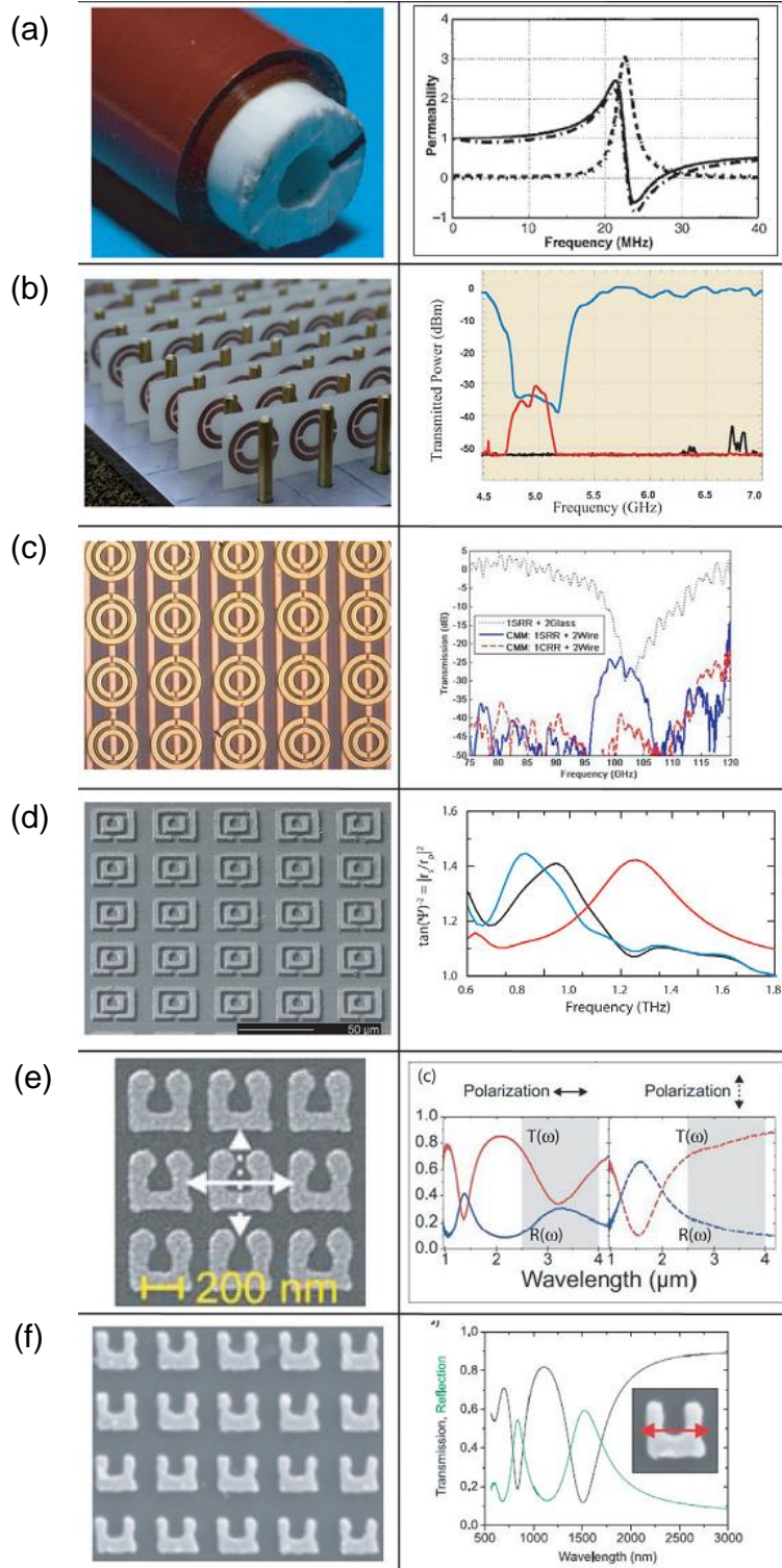
Figure 4-6 Metamaterial variations [89]
