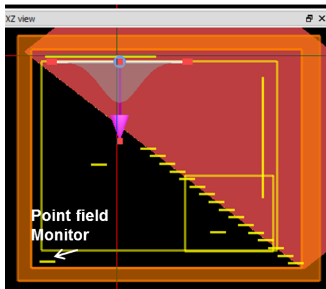
Figure 7-13 Lumerical FDTD simulation model showing the XZ plane view.
