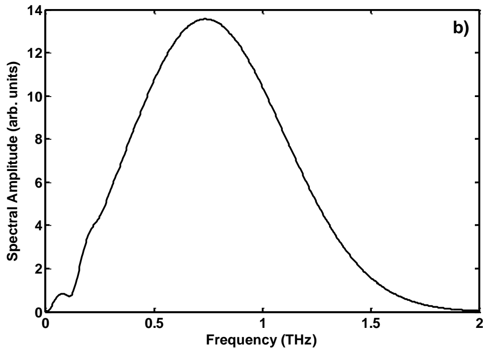
Figure 7-17 a) Spectra corresponding to time signals from Figure 7-16. b) Input spectrum.
