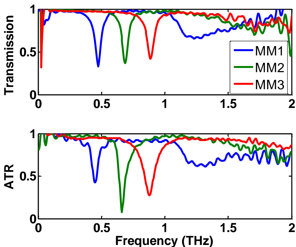
Figure 6-13 Measured transmission coefficient (top panel) and ATR reflection coefficient for samples MM1, MM2 and MM3 (bottom panel).
