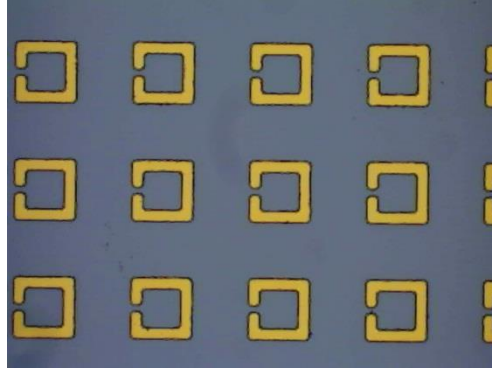
Figure 4-1 Sample array of square split ring resonators.
