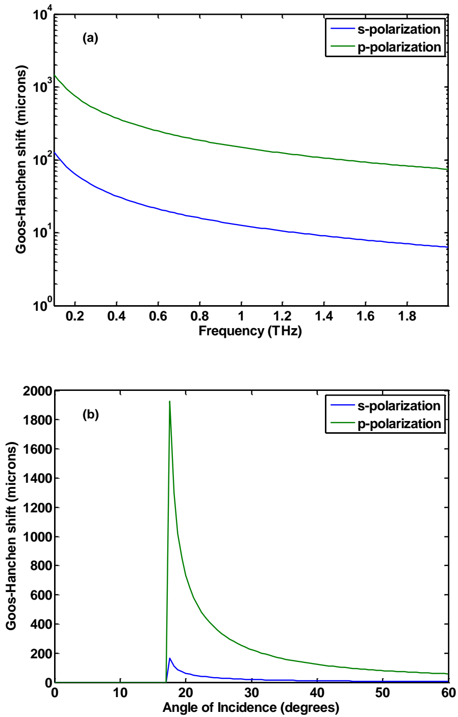
Figure 3-10 Goos-Hanchen shifts for s-polarization (blue) and p-polarized waves (green) plotted as a function of a) frequency for \theta_i = 45^\circ and b) incidence angle for a frequency of 1 THz.
