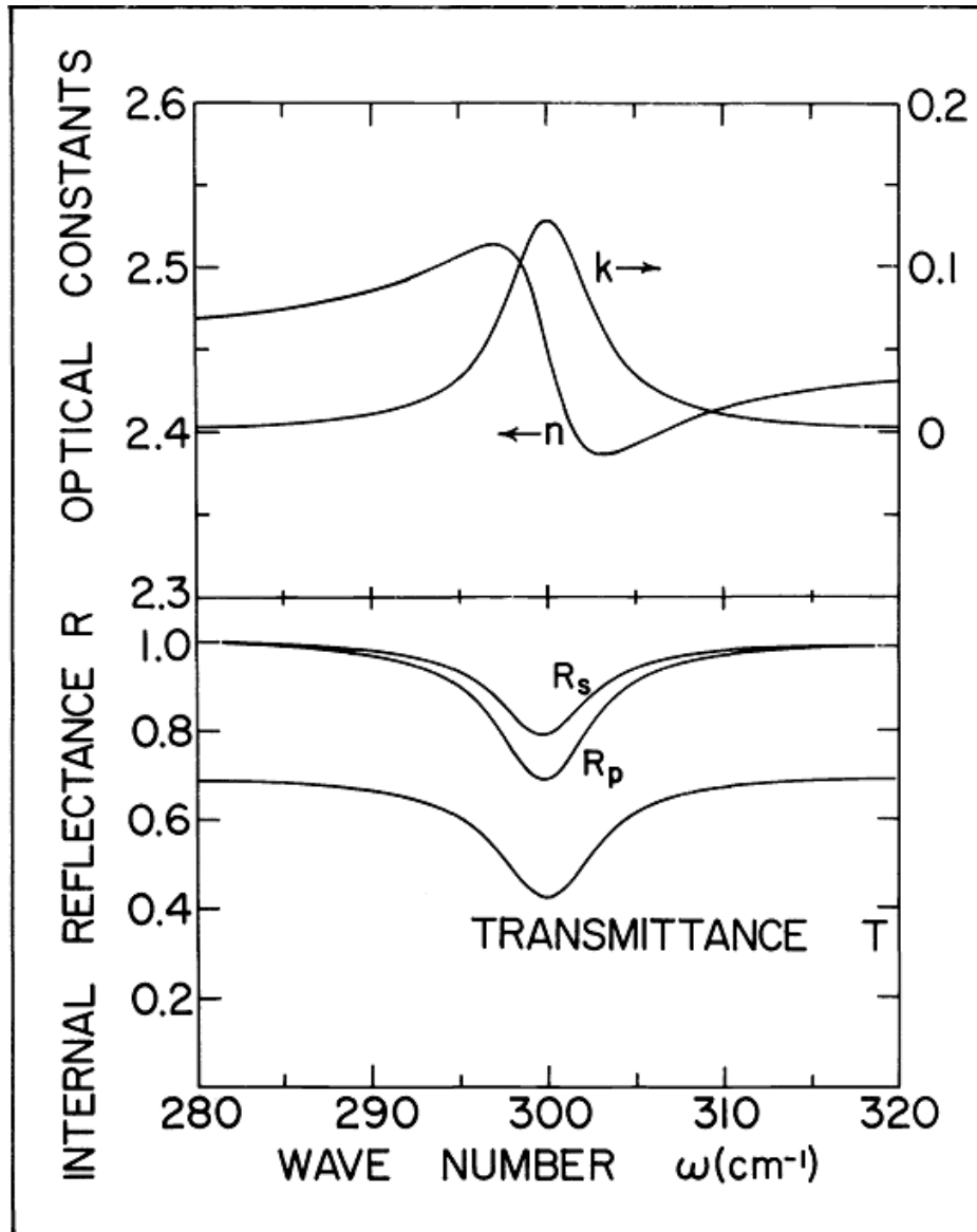
Figure 3-8 “Optical constants (refractive index n and extinction coefficient); (b) Internal- reflectance spectra for s and p polarization for a sample with optical constants shown in (a). The transmittance T for a 10 \mu\text{m} thick sample is also shown.” [71].
