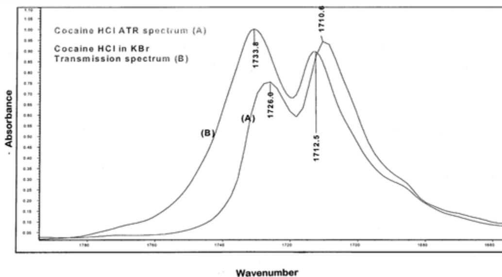
Figure 3-7 “The carbonyl band absorption of cocaine HCl showing the difference between ATR and absorbance spectra” [13]
