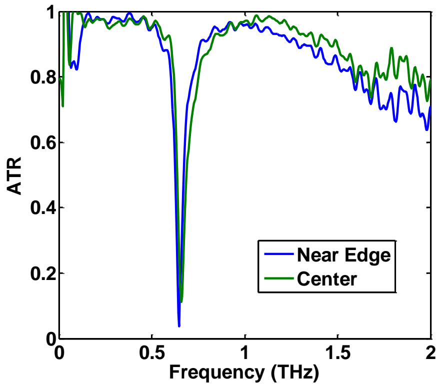
Figure 6-9: Measured ATR of MM2 for the edge (blue) and center (green) beam positions
