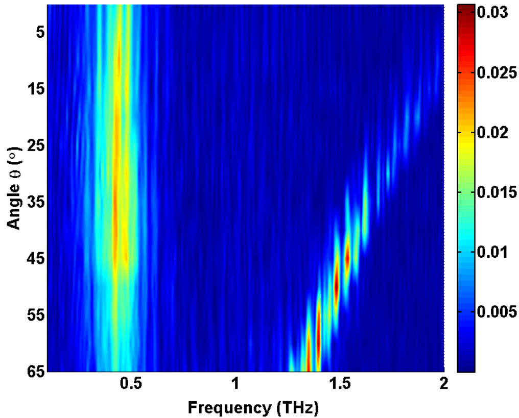
Figure 6-24: Angularly resolved spectra for radiation measurements from 0 to 65° from prism normal showing LC radiation and transmission grating signals.
