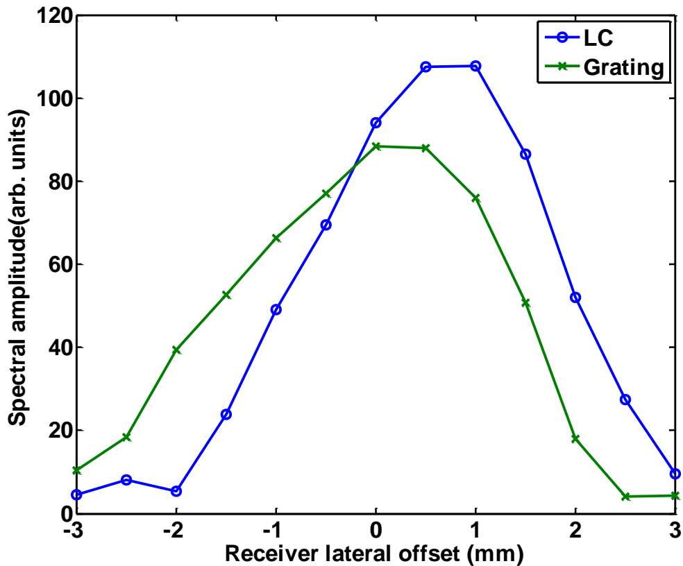
Figure 6-20: Edge excited beam profile measurements from re-radiation waveforms shown here for fundamental LC (blue) and the transmission grating (green) frequencies. Positive offset x is towards the edge and negative offsets x are toward the center of the array (see Figure 6-19).
