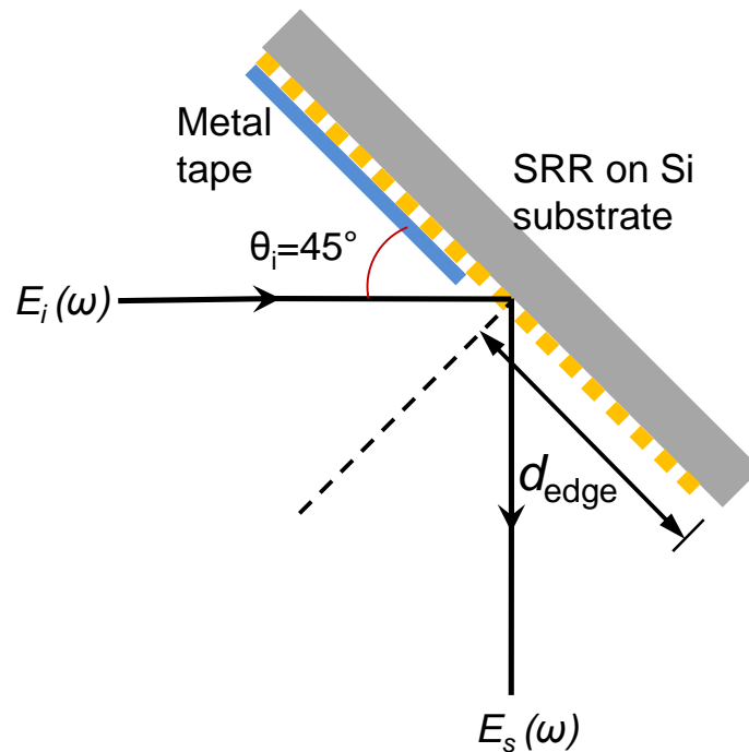
Figure 6-15: Arrangement for Reflection measurements at 45^\circ on sample MM1. Here d_{\text{edge}} indicates the relative displacement of the terahertz beam with respect to the edge of the array.
