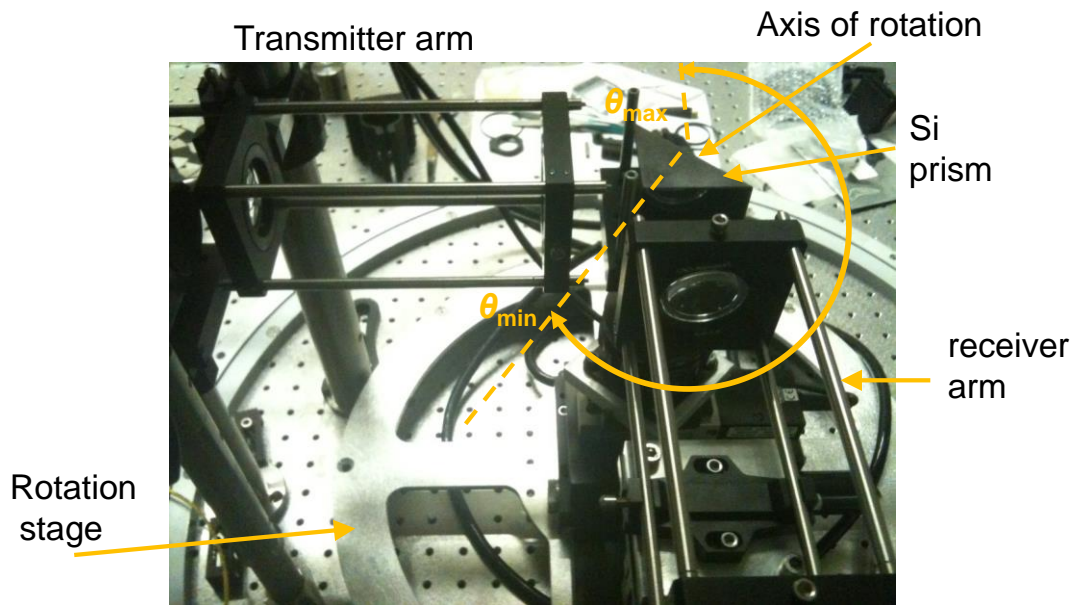
Figure 5-4 Transmitter and receiver arms cage system plus prism.
