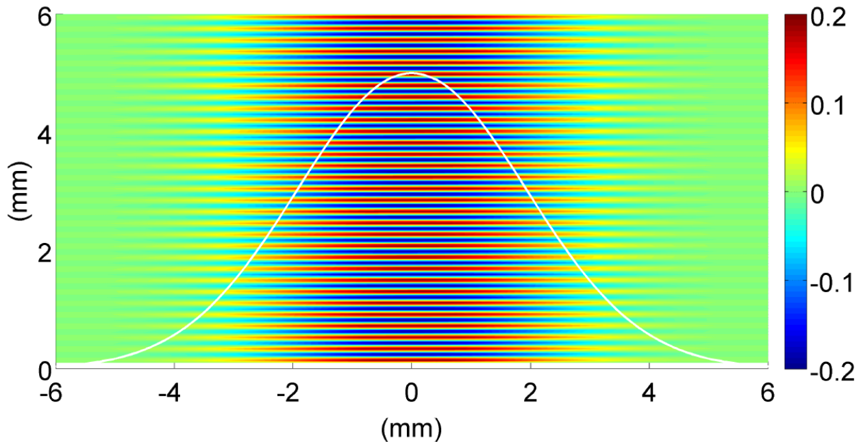
Figure 7-20 Electric field amplitude corresponding to s-polarization at the grating transmission frequency of 1.55 THz corresponding to a 0^\circ diffracted angle at the TIR boundary, for a wire array . No inter-element coupling is explicitly included in this treatment. The incident terahertz beam is shown in white[107]
