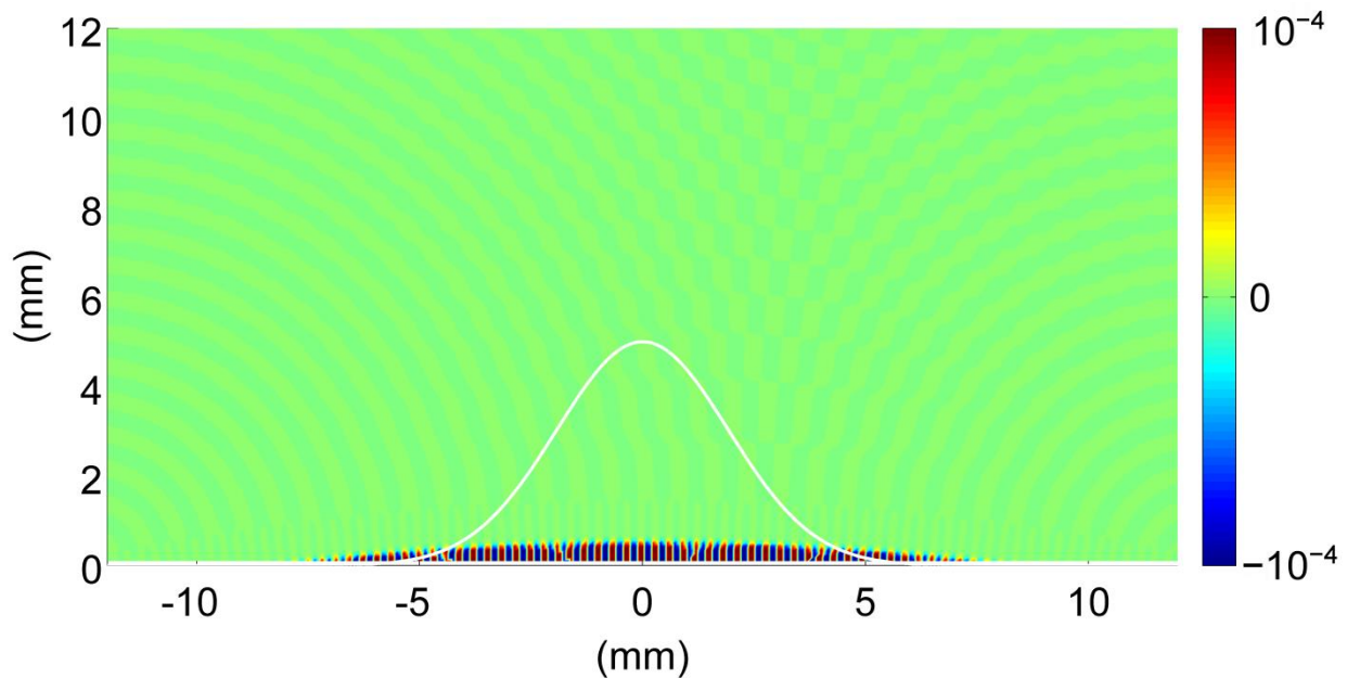
Figure 7-19 Electric field amplitude corresponding to s-polarization at the resonance frequency of 0.4 THz at the TIR boundary for a wire array that is 25 mm wide. No inter-element coupling is explicitly included in this treatment. The incident terahertz beam is shown in white.[107]
