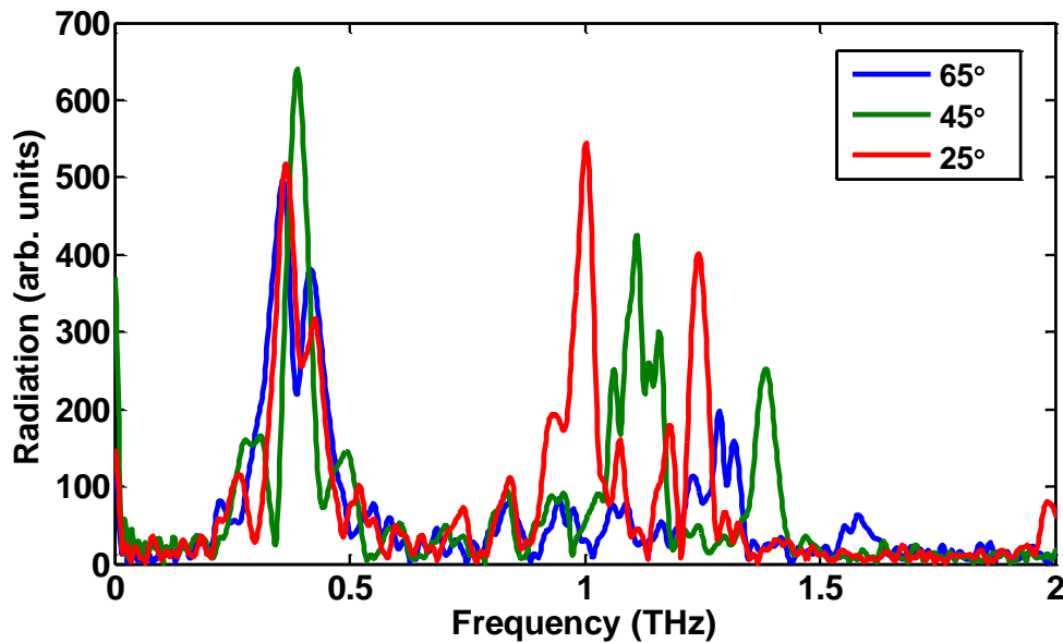
Figure 6-5 Angularly resolved spectra for re-radiation measurements at 25°, 45° and 65° from the optical axis, showing LC radiation and transmission grating signals.
