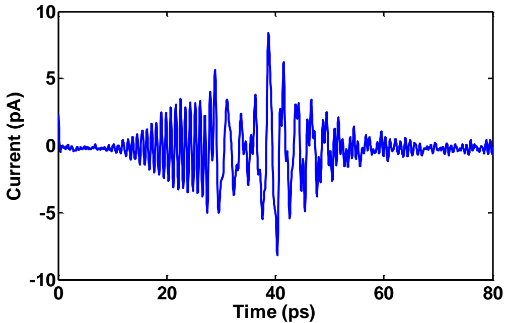
Figure 6-4 Re-radiation signal from a 1 cm 2 metafilm array.
