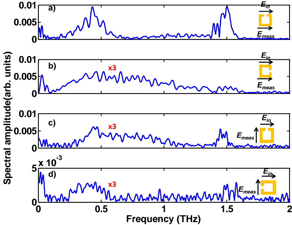
Figure 6-27 : Re-radiation spectra for different orientations of the SRR and detector. Incident field is p-polarized.
