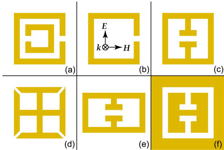
Figure 4-5 : Planar SRR topologies from [84]. “(a) single gap double resonator (b) single gap single loop, (c) electric LC resonators or eSRR, (d) four-fold rotational-symmetry eSRR, (e) rectangular eSRR and (f) complementary eSRR”.
