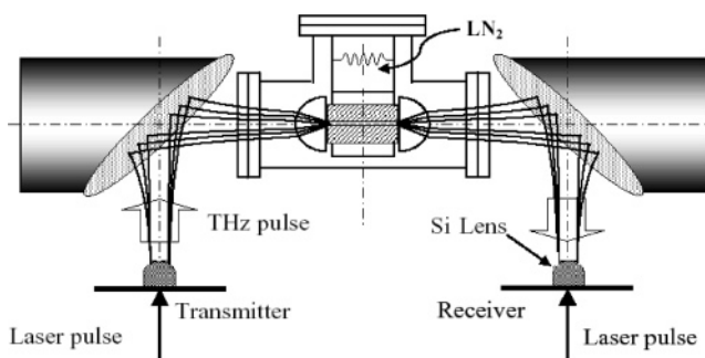
Figure 2. Schematic of the experimental apparatus for waveguide THz-TDS.
