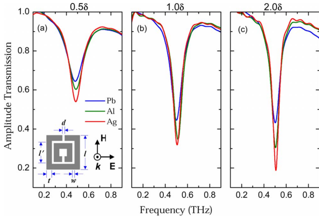
Fig. 1. (Color online) Measured frequency-dependent amplitude transmission of planar double SRR metamaterials made from Pb, Al, and Ag with various film thicknesses: (a) 0.5\delta , (b) 1.0\delta , and (c) 2.0\delta , near the LC resonance. Inset, schematic of the double SRR unit with dimensions w = 3 \mu\text{m} , metal width t = 6 \mu\text{m} , l = 36 \mu\text{m} , effective length of the SRR unit l' = 21 \mu\text{m} , d = 2 \mu\text{m} , and the periodicity P = 50 \mu\text{m} .
