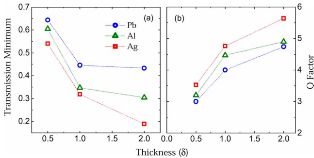
Fig. 2. (Color online) (a) Measured amplitude transmission minima and (b) Q factor at the LC resonance 0.5 THz for different metal SRRs with various thicknesses in skin depth.
