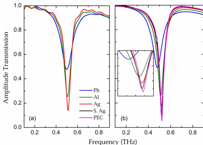
Fig. 4. (Color online) (a) THz-TDS results and (b) finite-element simulations of the LC resonant transmission of metamaterials made from 300 nm thick Pb, Al, Ag, S. Ag, and PEC. Inset, blow off of the simulated LC resonance.
