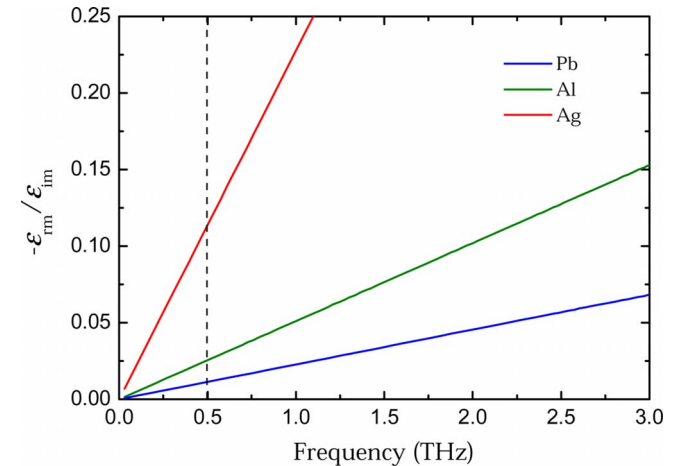
Fig. 3. (Color online) Frequency-dependent Drude ratio, -\epsilon_{rm}/\epsilon_{im} of Pb, Al, and Ag in the terahertz regime [11,12]; the vertical dashed line indicates the LC resonance frequency 0.5 THz.
