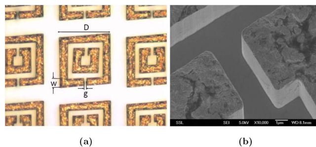
FIG. 1. (Color online) Optical (a) and scanning electron (b) micrographs of the gold SRRs fabricated for this work. The dimensions of the SRR are approximately D=38 \mu\text{m} , w=6 \mu\text{m} , and g=2 \mu\text{m} . The unit cell length is 50 \mu\text{m} .
