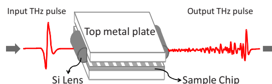
FIG. 1. (Color online) Cross-sectional view of the PPWG assembly together with the sample chip.
