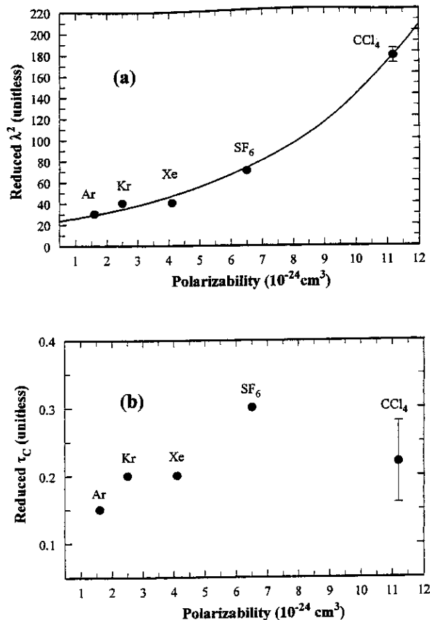
Figure 6. (a) The solute-solvent interaction strength plotted against the solvent polarizabilities for the symmetric series of solvents. The solid line denotes a NLLS quadratic fit ( R^2 = 0.99 ) to the data. (b) The correlation time of the anisotropic potential plotted against the solvent polarizability.
