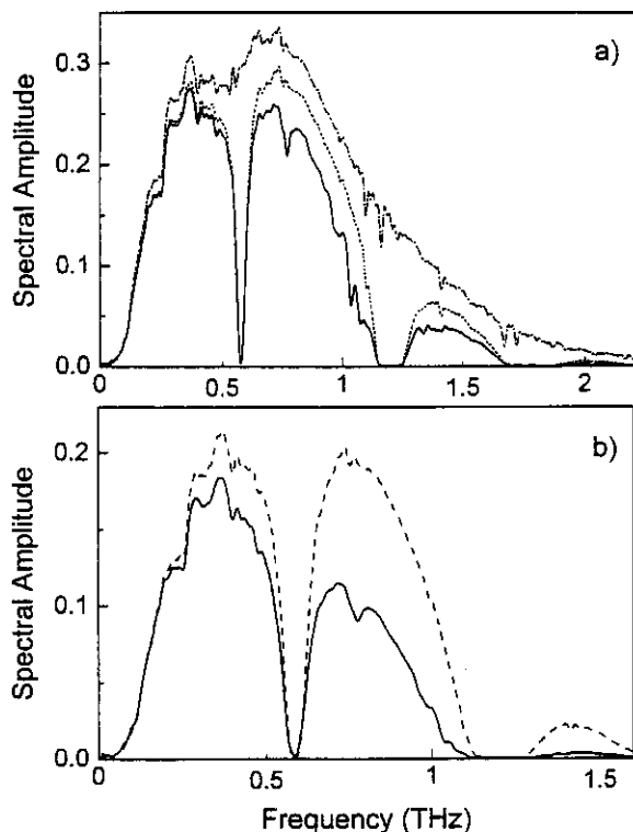
Figure 4. (a) Fourier transform spectrum of the transmitted THz pulse through a 380 mm long gas cell filled with 1000 hPa of ammonia vapor (lower solid line), the respective simulation for a pulse neglecting the additional absorption (middle dotted curve) and reference spectrum (upper dash-dotted line). (b) Fourier transform spectrum of a pulse transmitted through 2000 hPa ammonia vapor (solid line) and respective calculation without additional absorption (dashed line).
