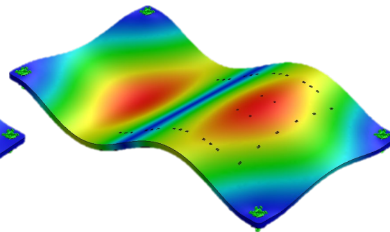
Figure 5: Mode Shape 3
