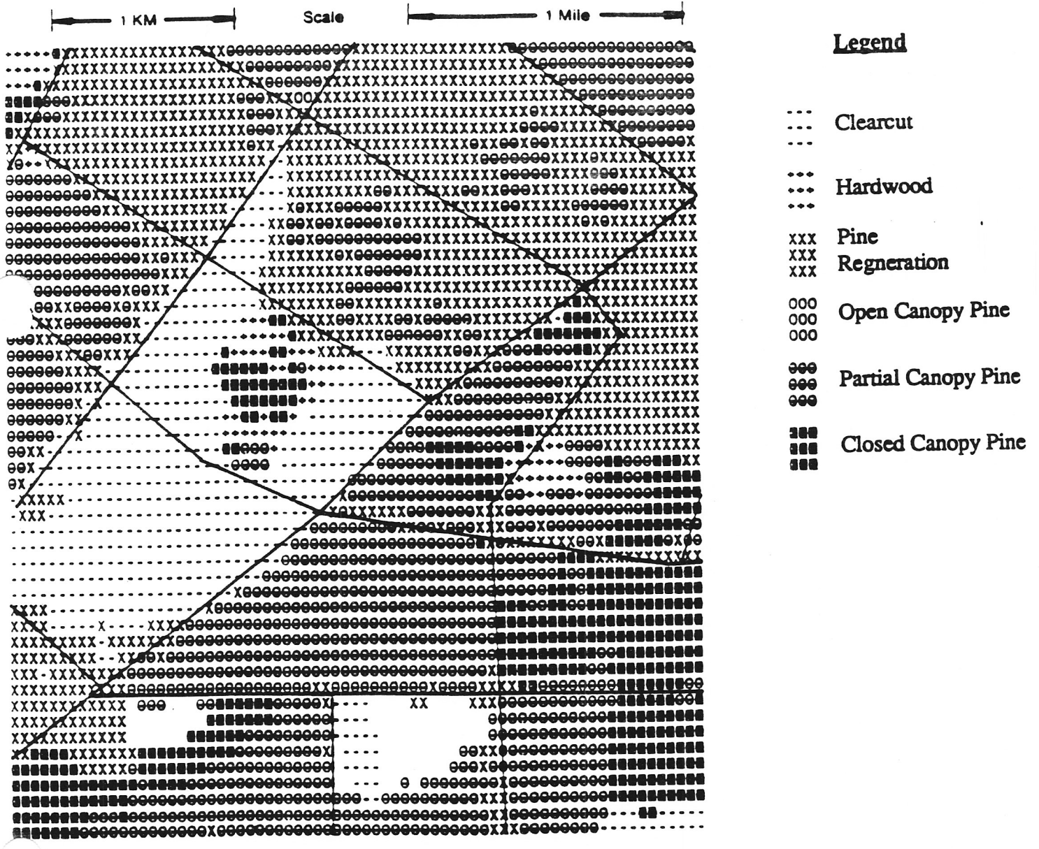
Figure 1. Computer generated map which illustrates the use of Landsat data in forest management.
